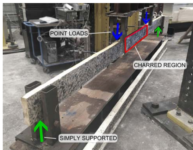
Figure 4: Mechanical loading of simply supported beam with two point loads. The beam in this image was charred in the centre, the region of high moment.
