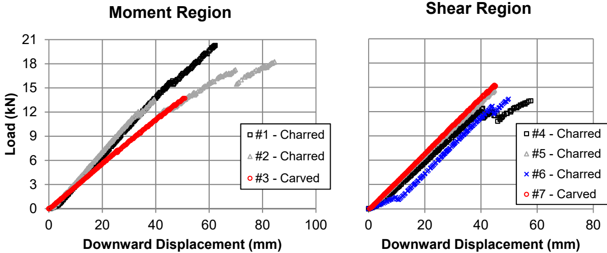
Figure 5: Load versus downward displacement of the carved and charred beams that have been damaged in the moment region (left) and shear region (right)
