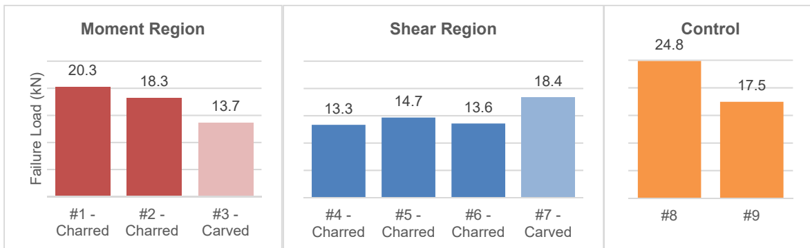
Figure 6. Comparison of the failure load of all beams damaged in the moment region, shear region, as well as the control beams
