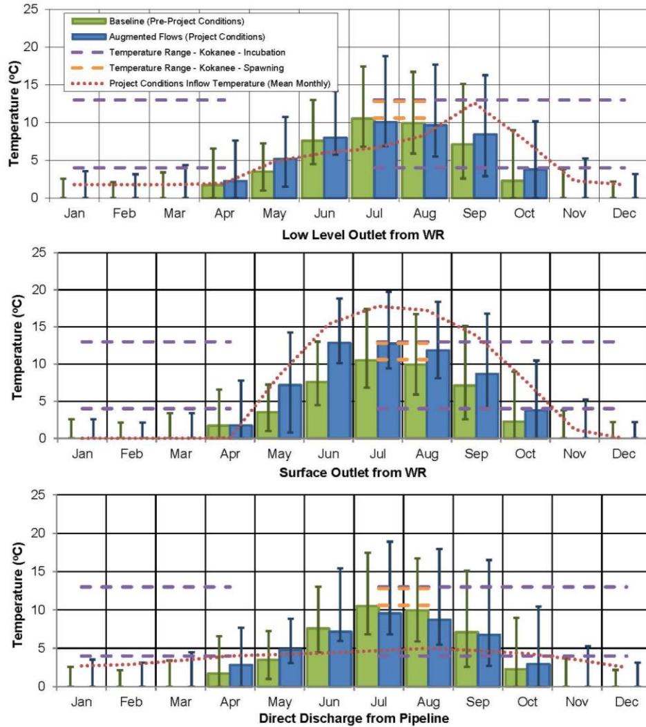
Figure 7: Simulated Creek water temperatures at kokanee habitat location
