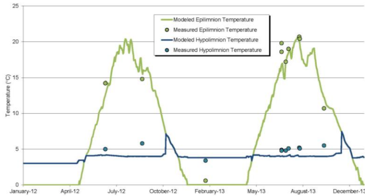
Figure 2: Temperature calibration of the Lake model.
