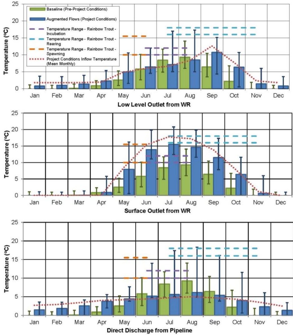
Figure 6: Simulated Creek water temperatures at rainbow trout habitat location
