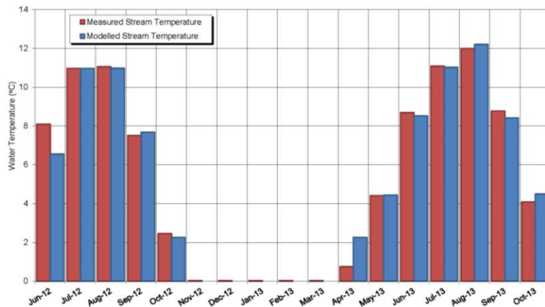
Figure 3: Temperature calibration of the Creek model.
